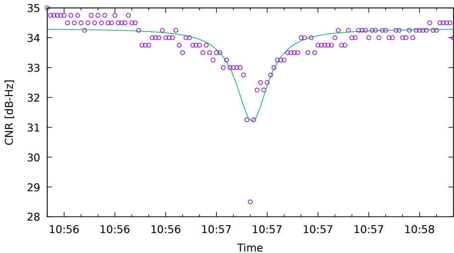
CNR fit for C09 on XiaomiMi8 - drive 10 (DOY263)
