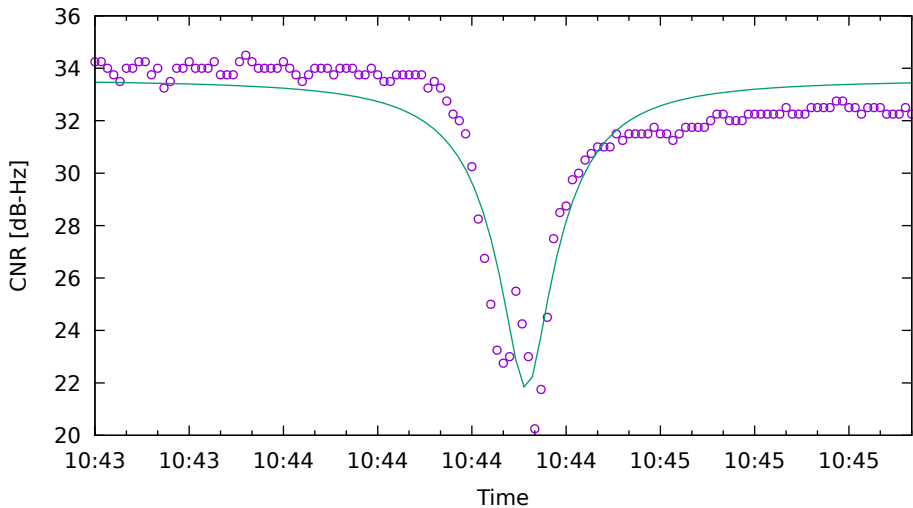
CNR fit for C09 on XiaomiMi8 - drive 3 (DOY263)
