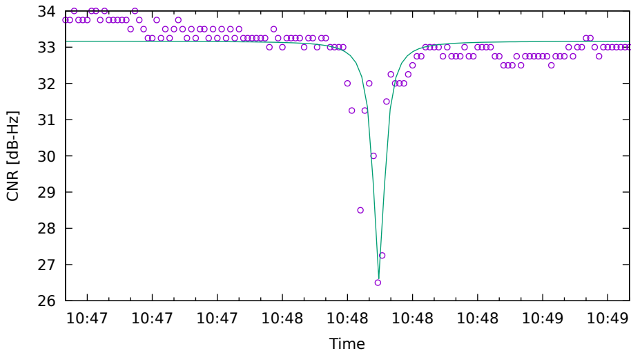
CNR fit for C09 on XiaomiMi8 - drive 5 (DOY263)
