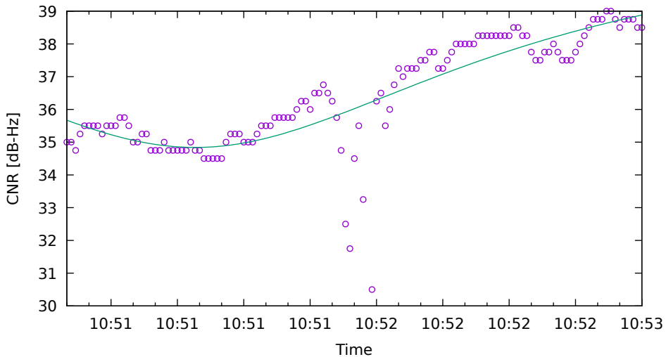
CNR fit for C21 on XiaomiMi8 - drive 7 (DOY263)
