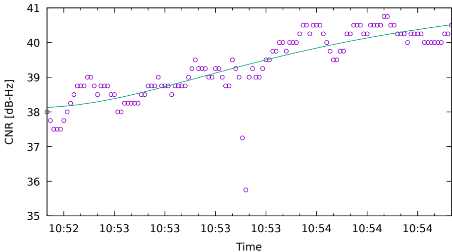
CNR fit for C21 on XiaomiMi8 - drive 8 (DOY263)
