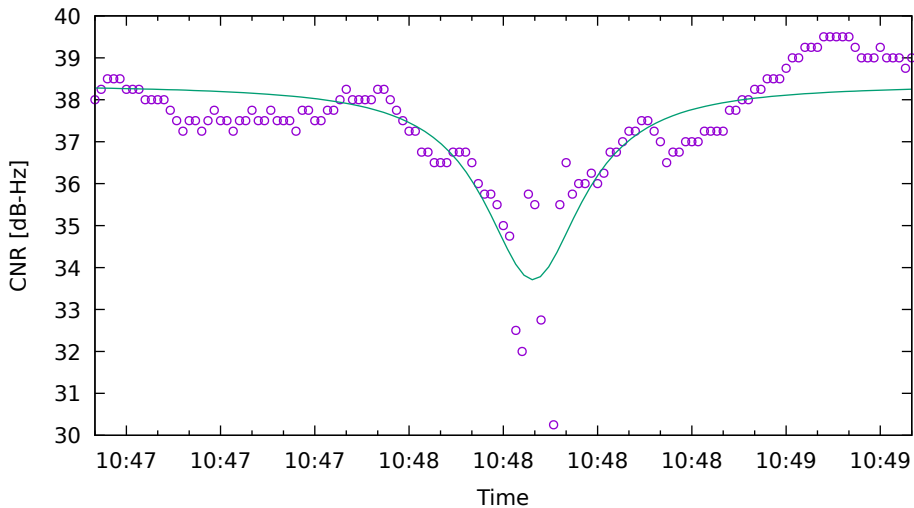
CNR fit for C26 on XiaomiMi8 - drive 5 (DOY263)
