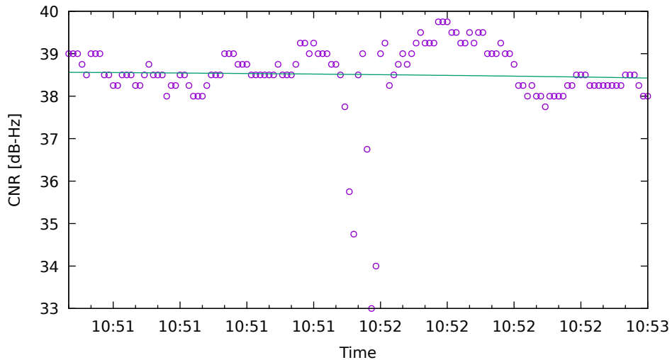
CNR fit for C26 on XiaomiMi8 - drive 7 (DOY263)
