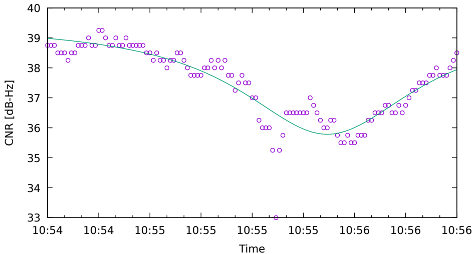
CNR fit for C26 on XiaomiMi8 - drive 9 (DOY263)
