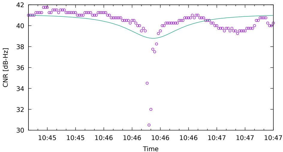
CNR fit for C28 on XiaomiMi8 - drive 4 (DOY263)
