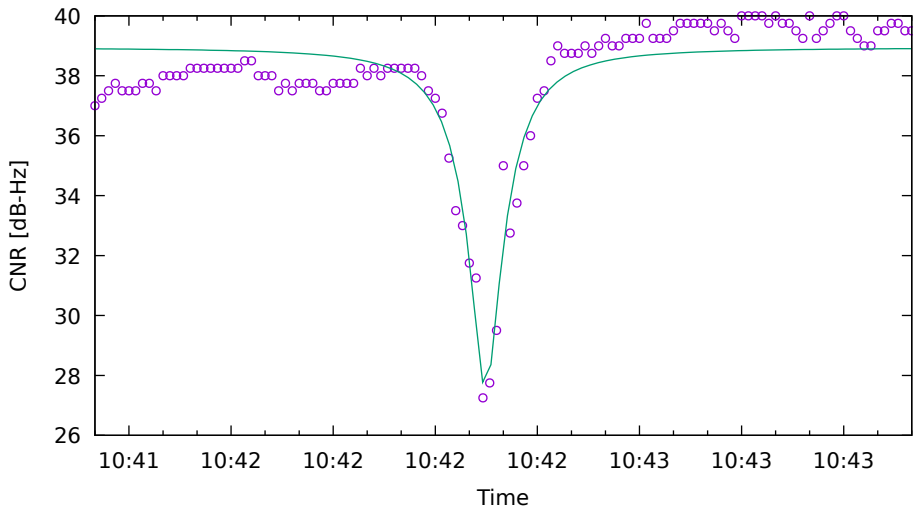
CNR fit for C33 on XiaomiMi8 - drive 2 (DOY263)
