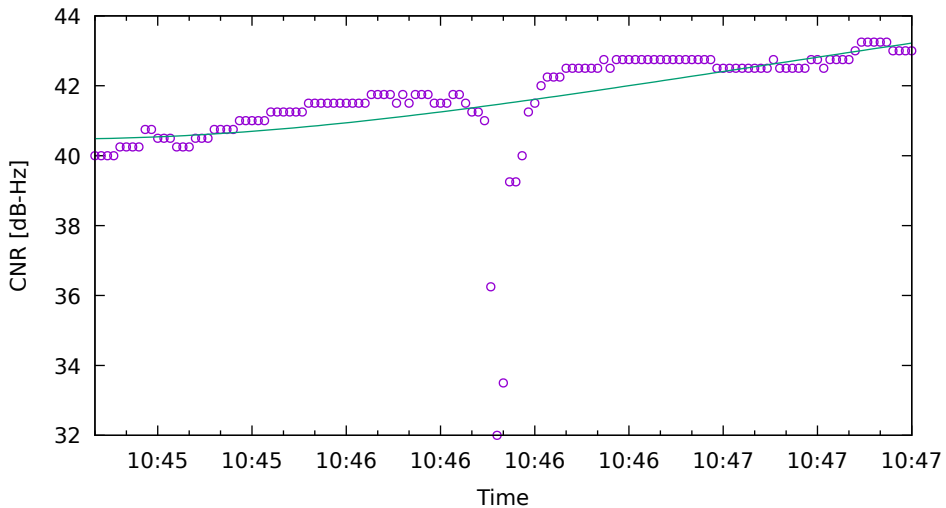
CNR fit for C33 on XiaomiMi8 - drive 4 (DOY263)
