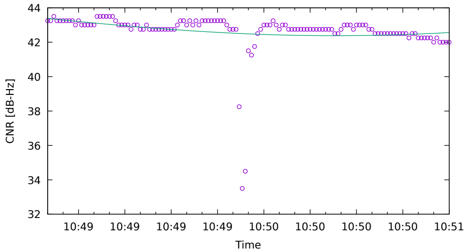
CNR fit for C33 on XiaomiMi8 - drive 6 (DOY263)
