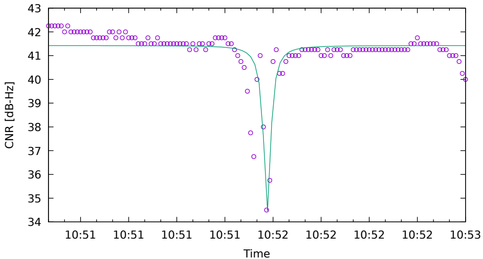
CNR fit for C33 on XiaomiMi8 - drive 7 (DOY263)
