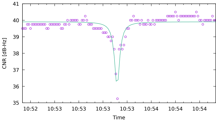
CNR fit for E04 on XiaomiMi8 - drive 8 (DOY263)
