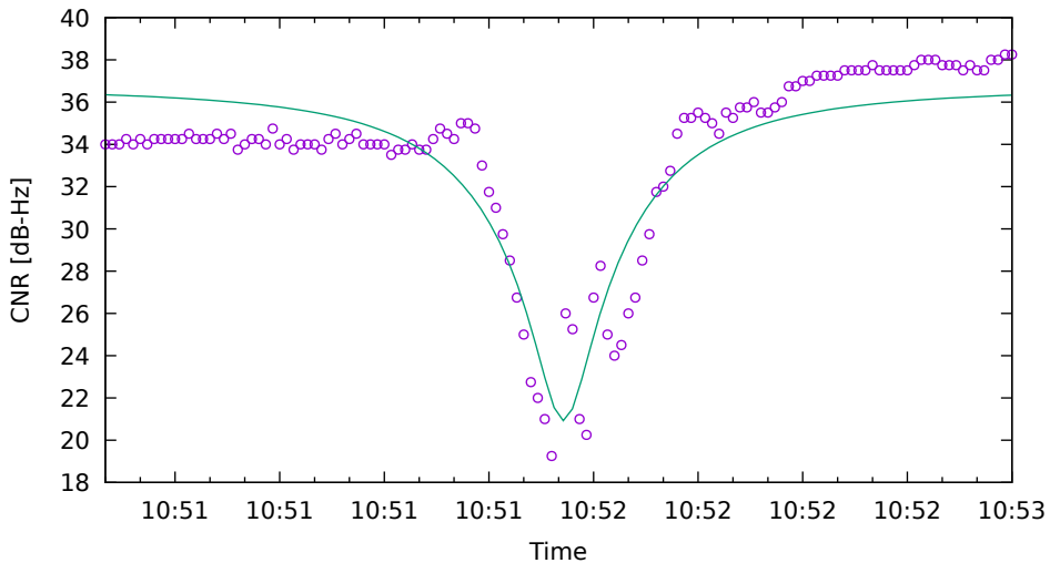
CNR fit for E33 on XiaomiMi8 - drive 7 (DOY263)
