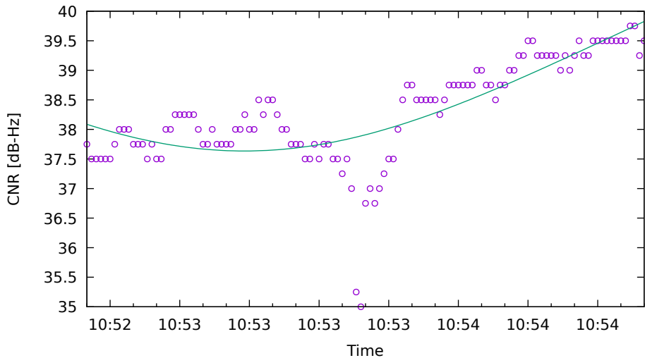
CNR fit for E33 on XiaomiMi8 - drive 8 (DOY263)
