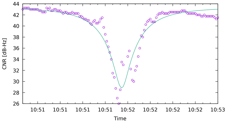
CNR fit for G01 on XiaomiMi8 - drive 7 (DOY263)
