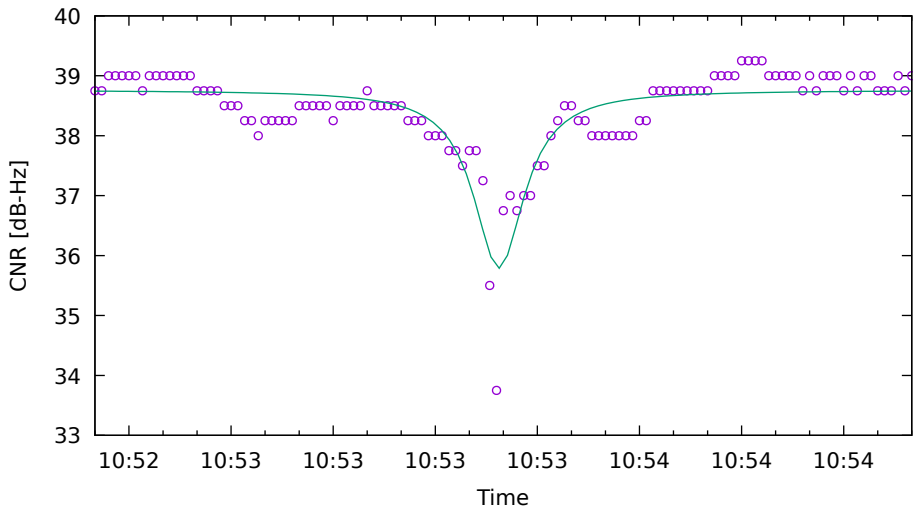
CNR fit for G04 on XiaomiMi8 - drive 8 (DOY263)
