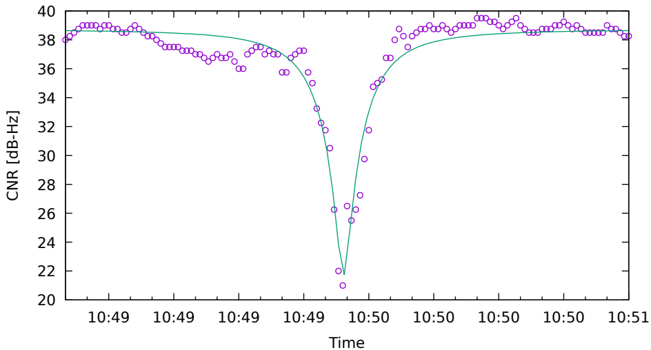
CNR fit for G17 on XiaomiMi8 - drive 6 (DOY263)
