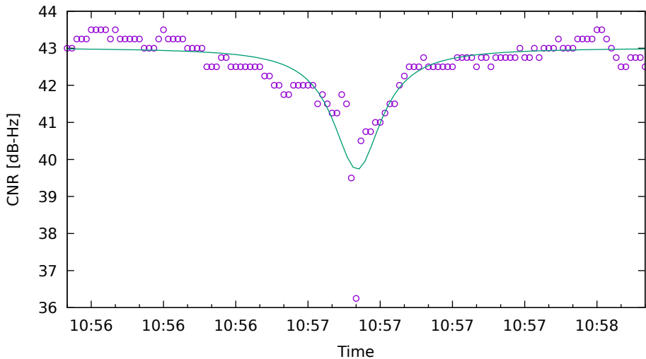
CNR fit for G19 on XiaomiMi8 - drive 10 (DOY263)
