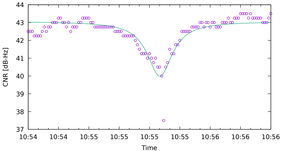
CNR fit for G19 on XiaomiMi8 - drive 9 (DOY263)
