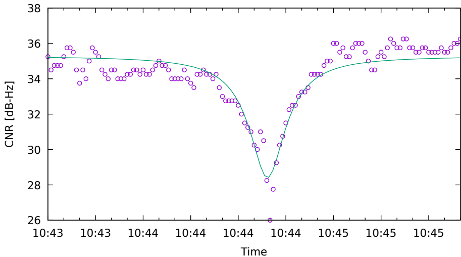
CNR fit for G22 on XiaomiMi8 - drive 3 (DOY263)
