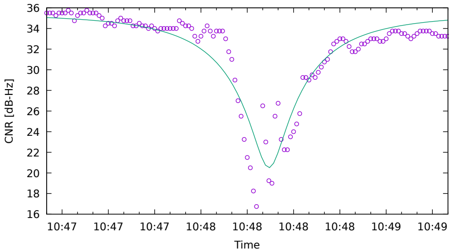
CNR fit for G22 on XiaomiMi8 - drive 5 (DOY263)
