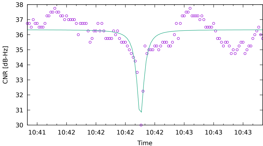
CNR fit for G31 on XiaomiMi8 - drive 2 (DOY263)
