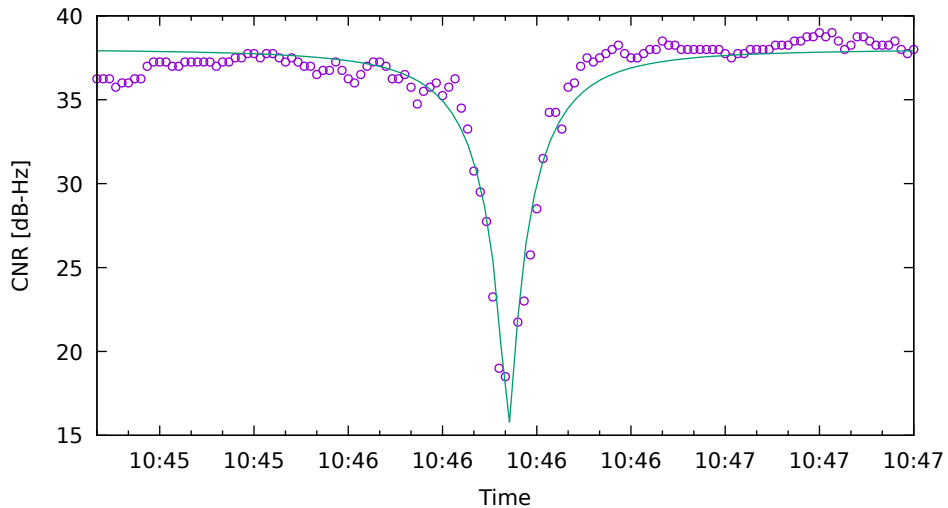
CNR fit for G31 on XiaomiMi8 - drive 4 (DOY263)
