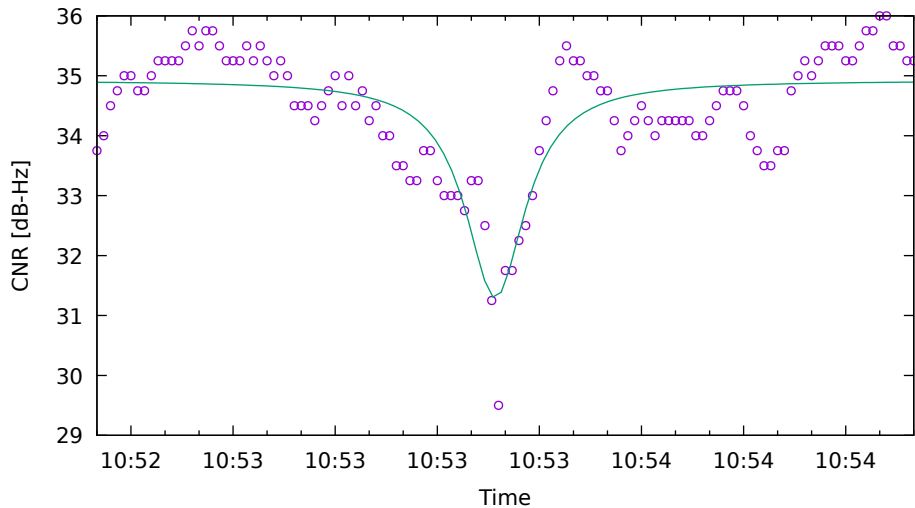
CNR fit for G31 on XiaomiMi8 - drive 8 (DOY263)
