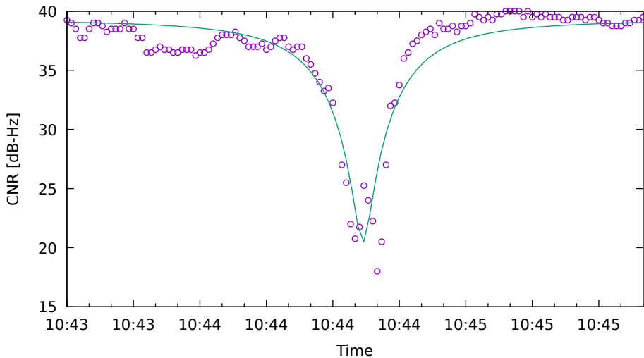
CNR fit for R02 on XiaomiMi8 - drive 3 (DOY263)
