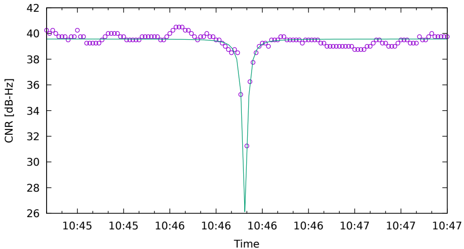
CNR fit for R17 on XiaomiMi8 - drive 4 (DOY263)
