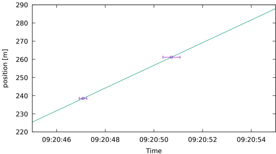
Jammer position fit DOY262 S1 drive 3
