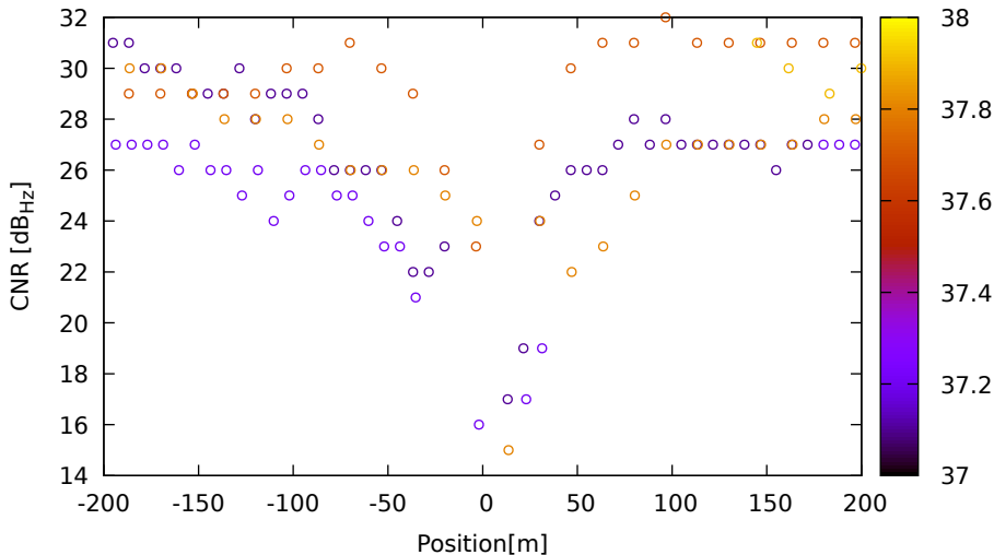
CNR vs position for C09 (B1) on HuaweiP40 - DOY 262 jam. 1
