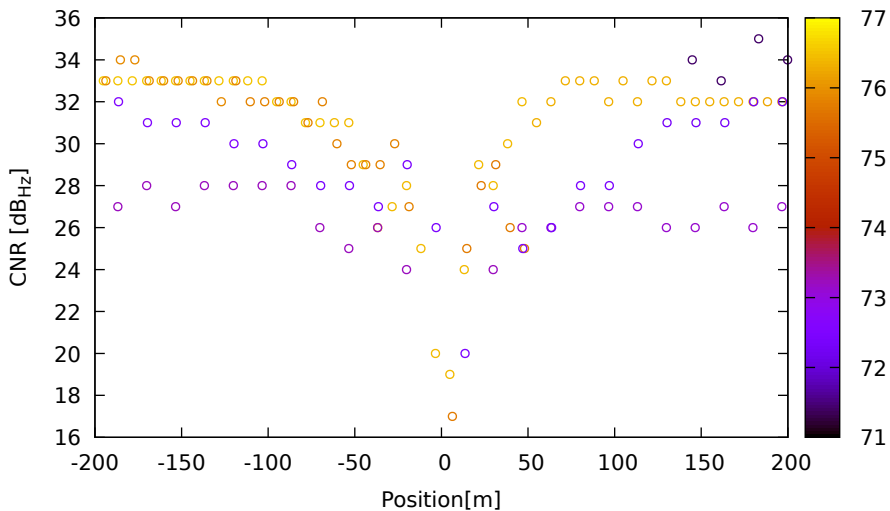
CNR vs position for C14 (B1) on HuaweiP40 - DOY 262 jam. 1
