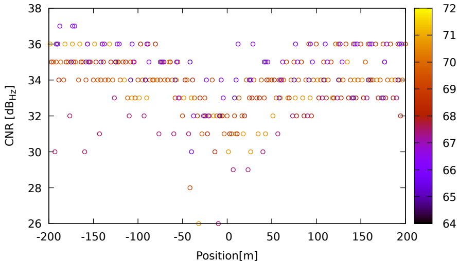
CNR vs position for C14 (B1) on HuaweiP40 - DOY 262 jam. 2
