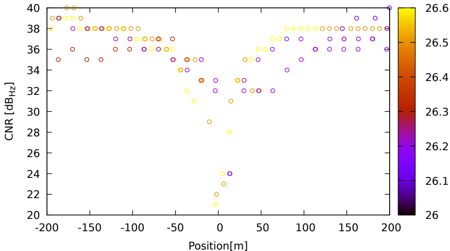
CNR vs position for C16 (B1) on HuaweiP40 - DOY 262 jam. 1
