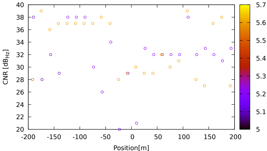
CNR vs position for C26 (B1) on HuaweiP40 - DOY 262 jam. 2
