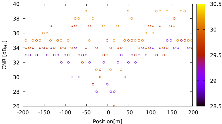
CNR vs position for C27 (B1) on HuaweiP40 - DOY 262 jam. 3
