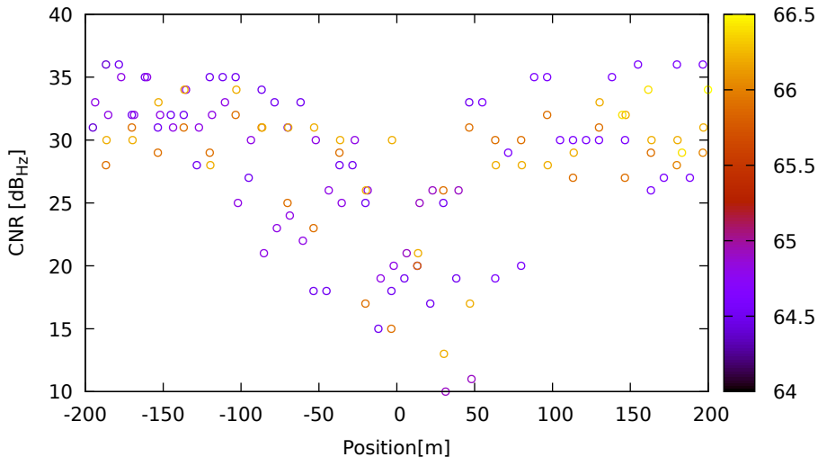
CNR vs position for C28 (B1) on HuaweiP40 - DOY 262 jam. 1
