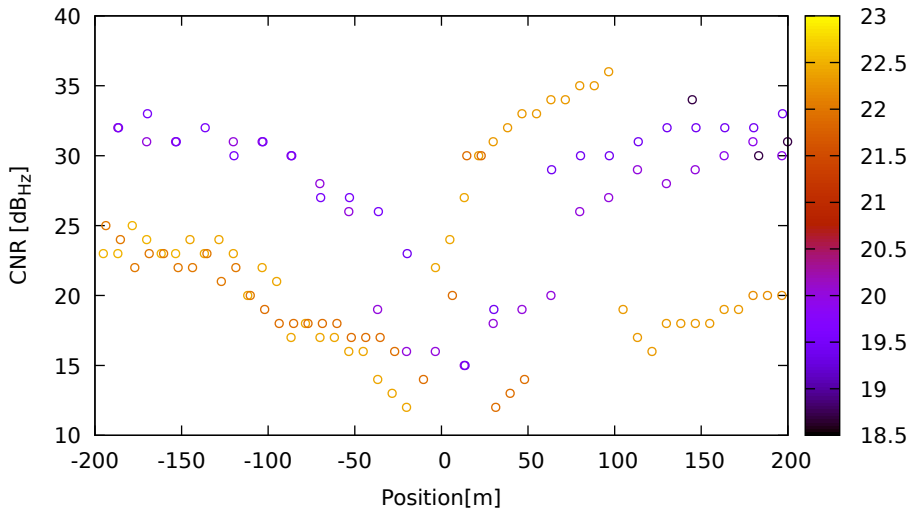
CNR vs position for E04 (E1) on HuaweiP40 - DOY 262 jam. 1
