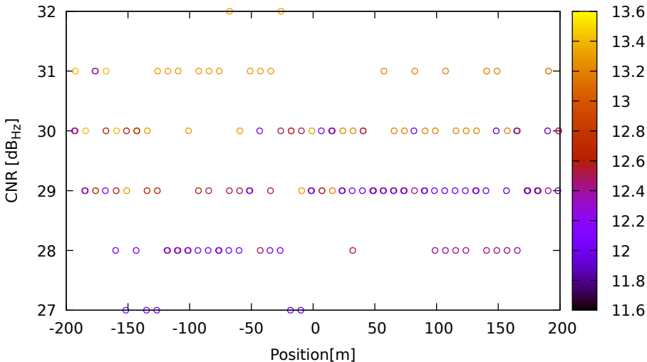
CNR vs position for E04 (E1) on HuaweiP40 - DOY 262 jam. 3
