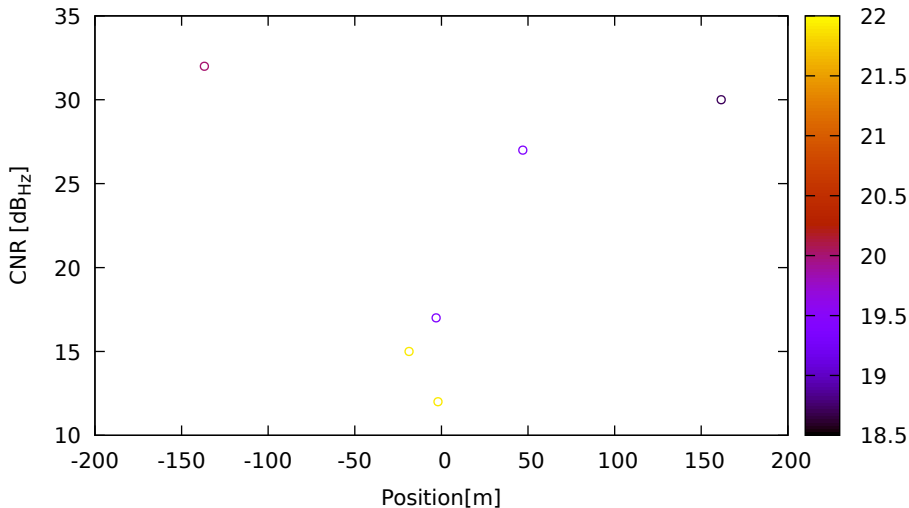
CNR vs position for E04 (E5a) on HuaweiP40 - DOY 262 jam. 1
