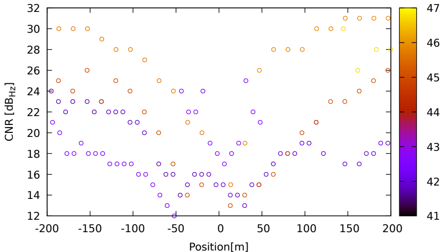
CNR vs position for E05 (E1) on HuaweiP40 - DOY 262 jam. 1
