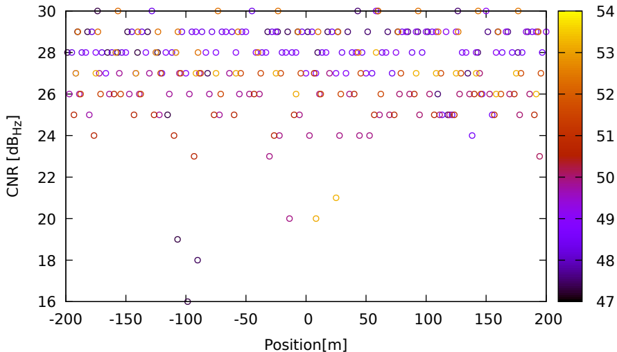
CNR vs position for E05 (E1) on HuaweiP40 - DOY 262 jam. 2
