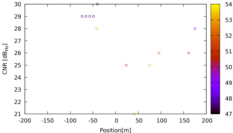
CNR vs position for E05 (E5a) on HuaweiP40 - DOY 262 jam. 2
