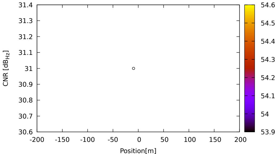
CNR vs position for E05 (E5a) on HuaweiP40 - DOY 262 jam. 3
