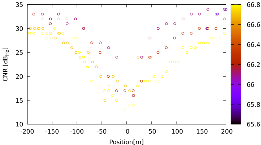
CNR vs position for E09 (E1) on HuaweiP40 - DOY 262 jam. 1
