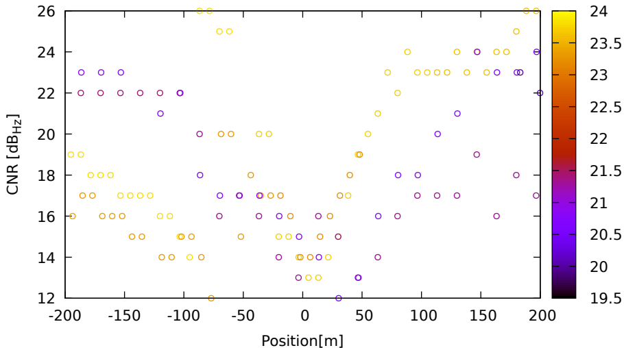
CNR vs position for E11 (E1) on HuaweiP40 - DOY 262 jam. 1
