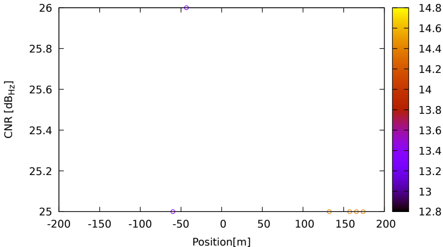
CNR vs position for E11 (E5a) on HuaweiP40 - DOY 262 jam. 3
