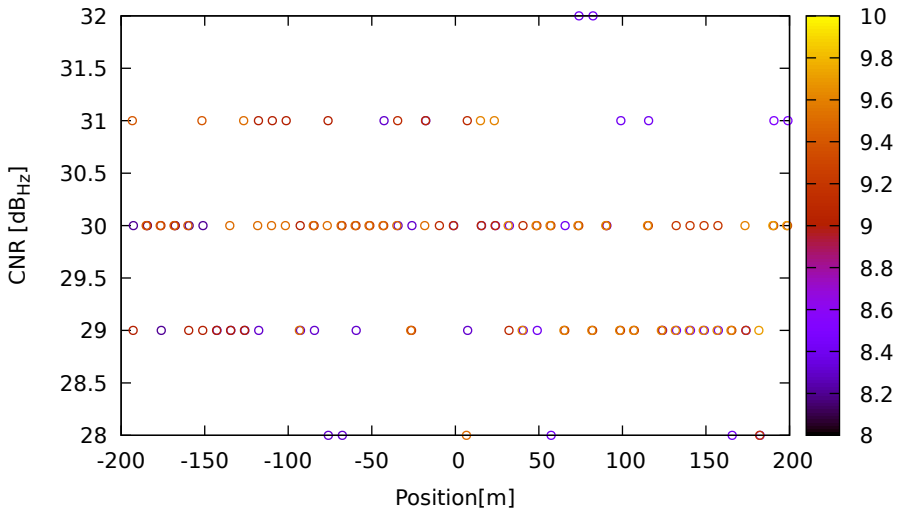
CNR vs position for E15 (E1) on HuaweiP40 - DOY 262 jam. 3
