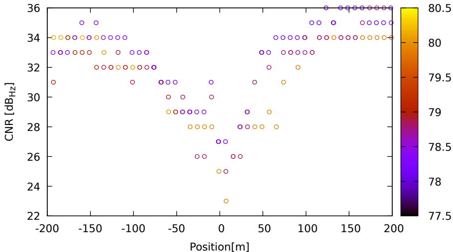
CNR vs position for G01 (L1) on HuaweiP40 - DOY 262 jam. 3
