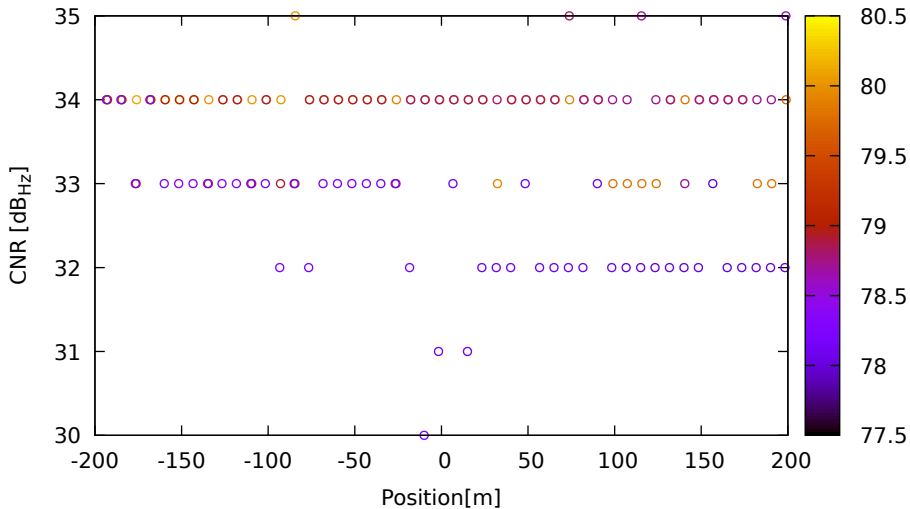
CNR vs position for G01 (L5) on HuaweiP40 - DOY 262 jam. 3
