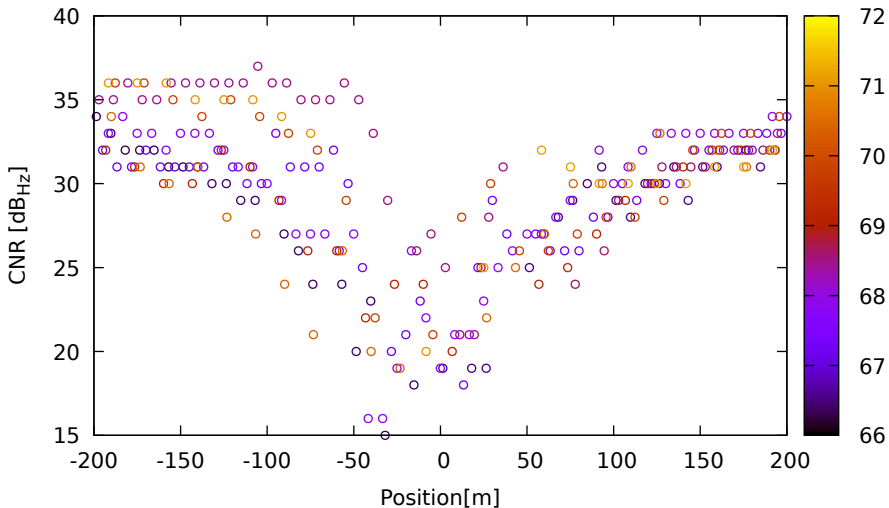
CNR vs position for G03 (L1) on HuaweiP40 - DOY 262 jam. 2
